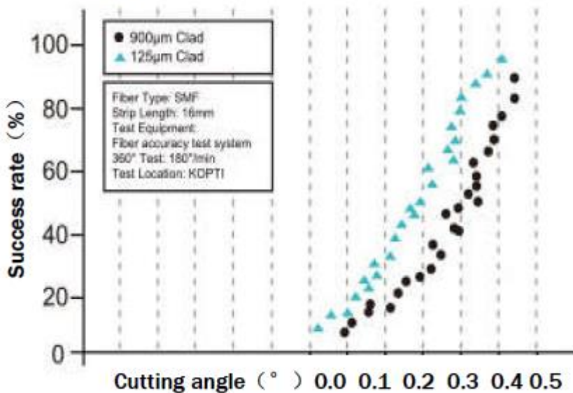
(Cutting angle test)
