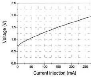
I-V Curve
