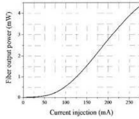
P-I Curve
