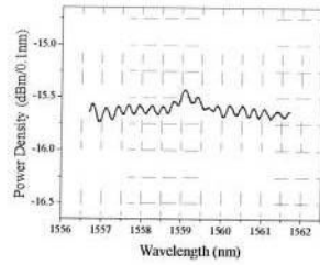
Spectrum Modulation
