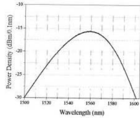
Spontaneous Emission Spectrum
