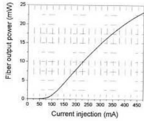
P-I Curve
