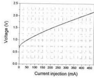
I-V Curve
