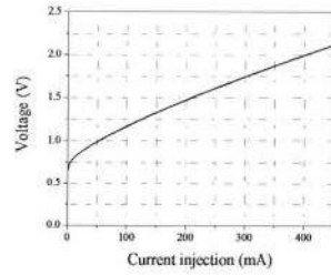
I-V Curve
