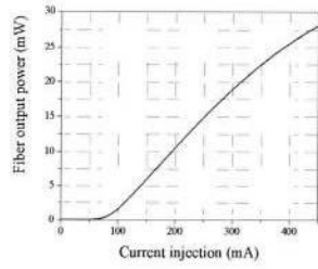
P-I Curve
