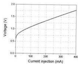
I-V Curve
