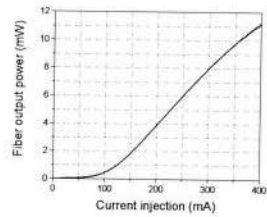
P-I Curve
