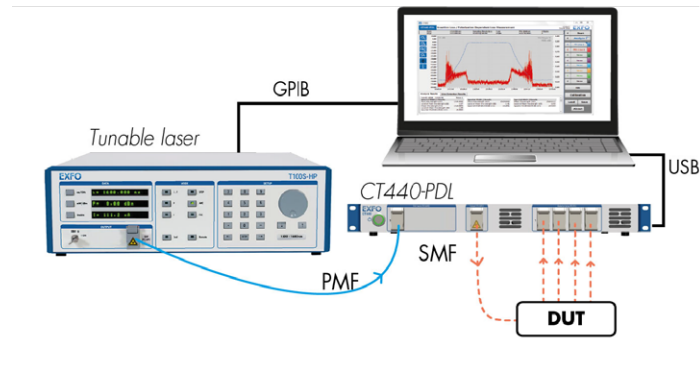
Figure 7. PDL measurement using the CT440-PDL
