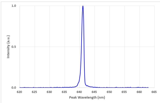
Figure 2 : Spectral Characteristics 光谱曲线
