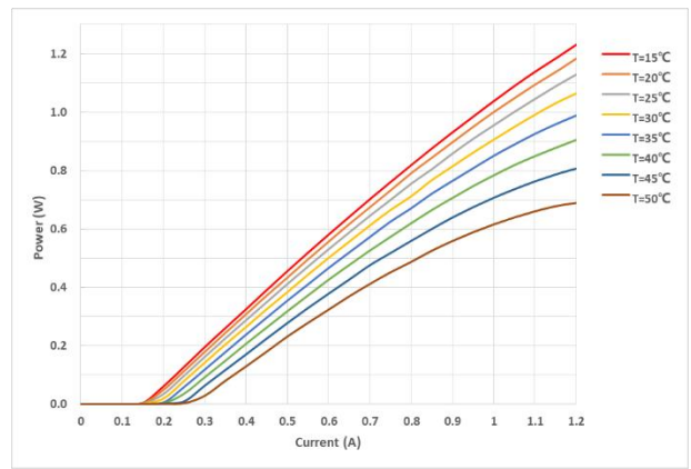
Figure 4 : Power-Current Curve at Different Temperature
