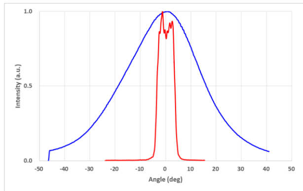
Figure 3 : Far Field Pattern Characteristics 远场发散角曲线
