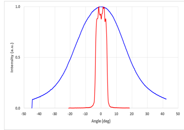
Figure 3 : Far Field Pattern Characteristics 远场发散角曲线
