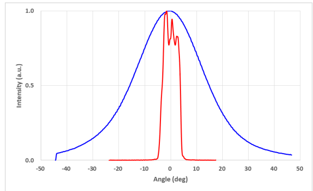
Figure 3 : Far Field Pattern Characteristics 远场发散角曲线
