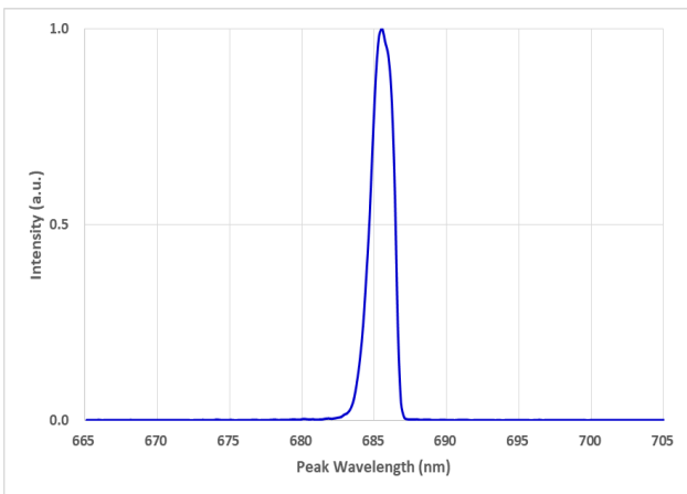
Figure 2 : Spectral Characteristics 光谱曲线
