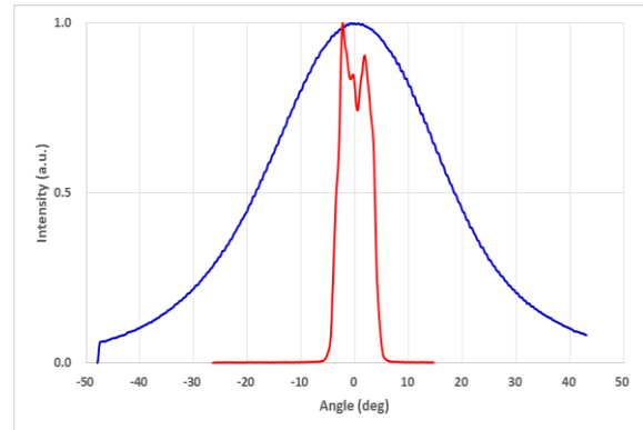
Figure 3 : Far Field Pattern Characteristics 远场发散角曲线
