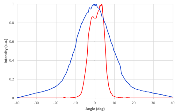
Figure 4 : Near Field Pattern (NFP)
